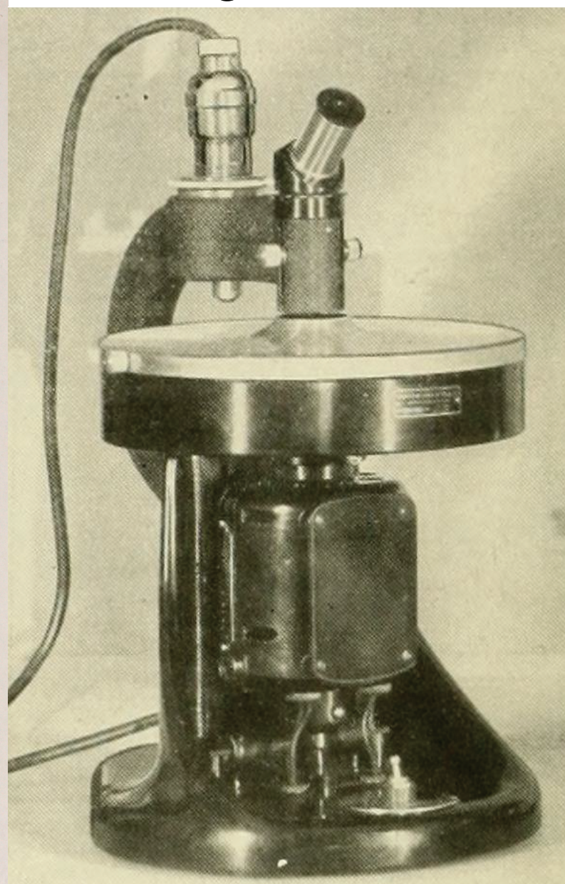
Optical centrifuge
